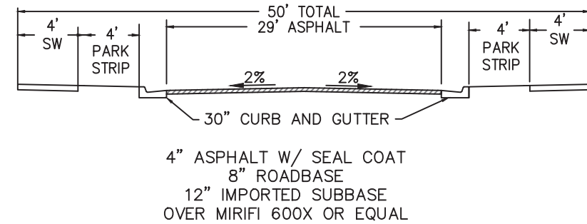
1450 W STREET CROSS SECTION
