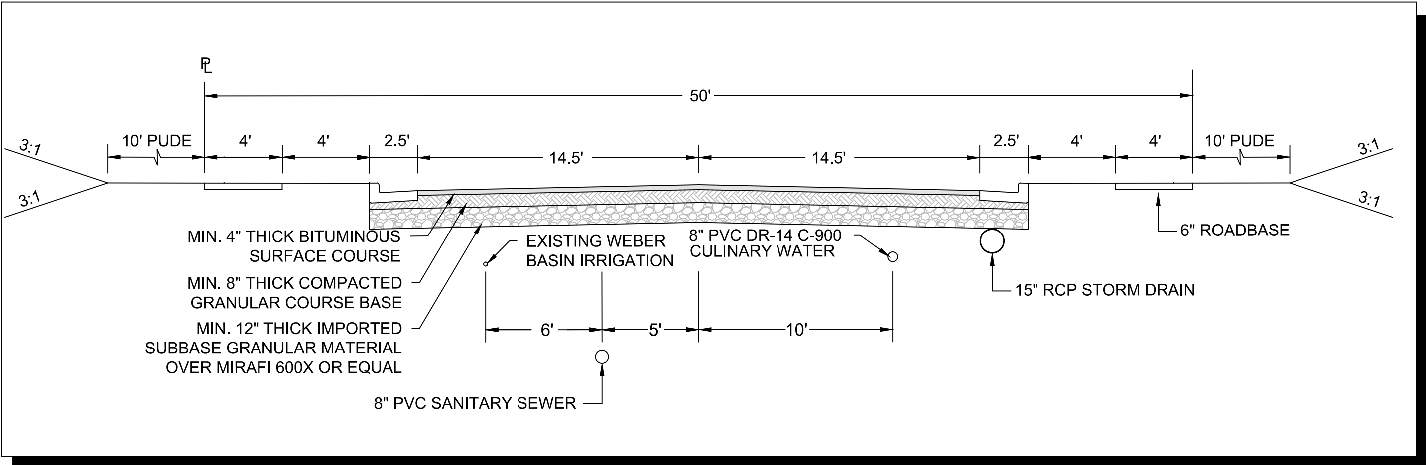
50' STANDARD CROSS SECTION
