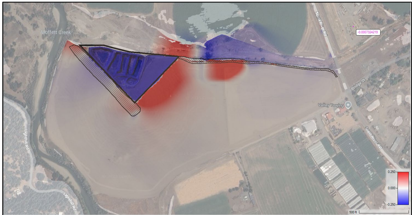
Figure 6. Model results (100-year event) for West Site showing maximum water surface elevation change from baseline conditions.
