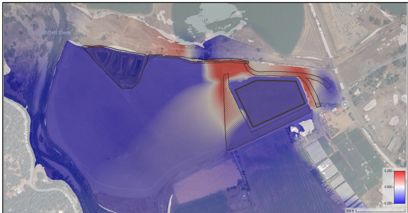
Figure 5. Model results (100-year event) for East Site showing maximum water surface elevation change from baseline conditions.
